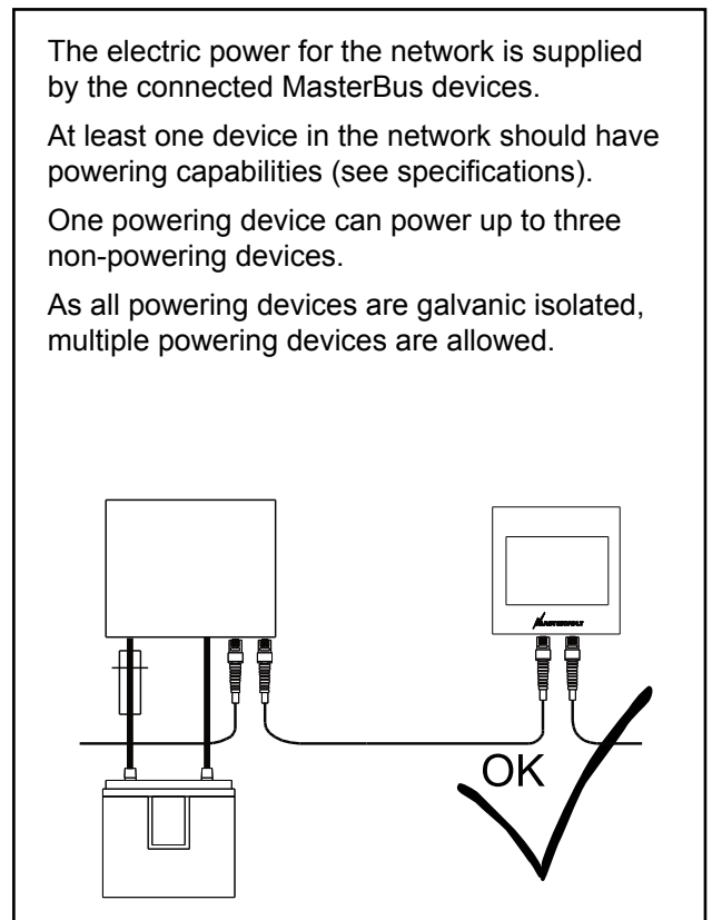
Figure 6: Power supply
