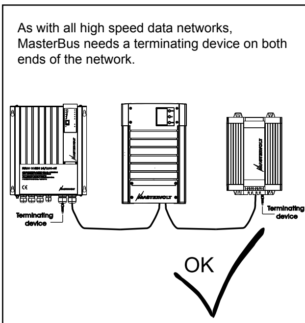
Figure 5: Two Terminators
