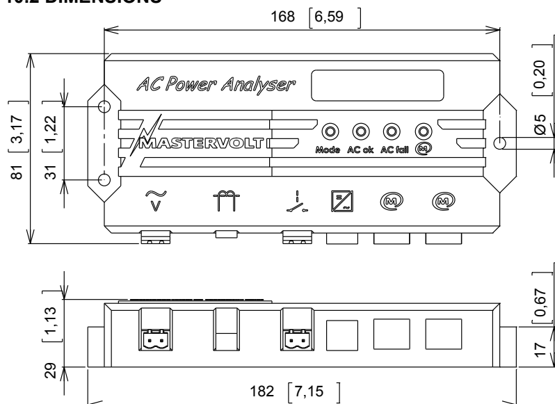
Figure 12: Dimensions in mm [inches]
