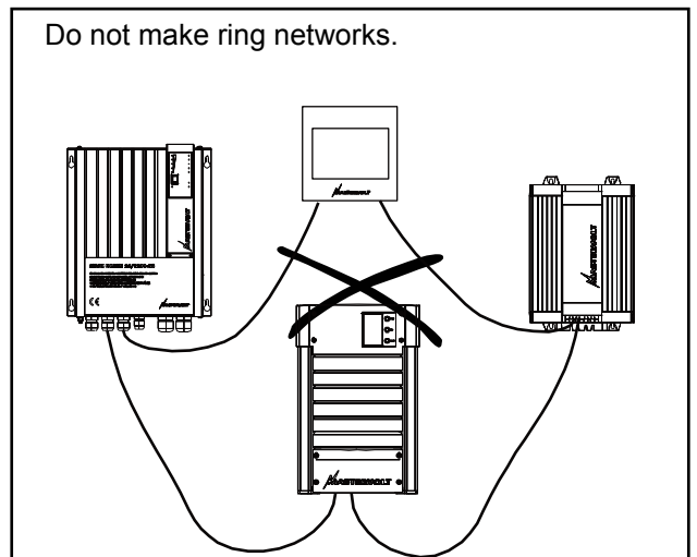
Figure 7: No ring networks
